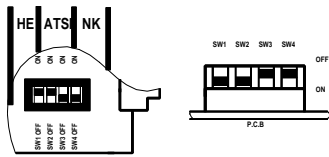
Microstep selector switches set to 3200 steps/rev
